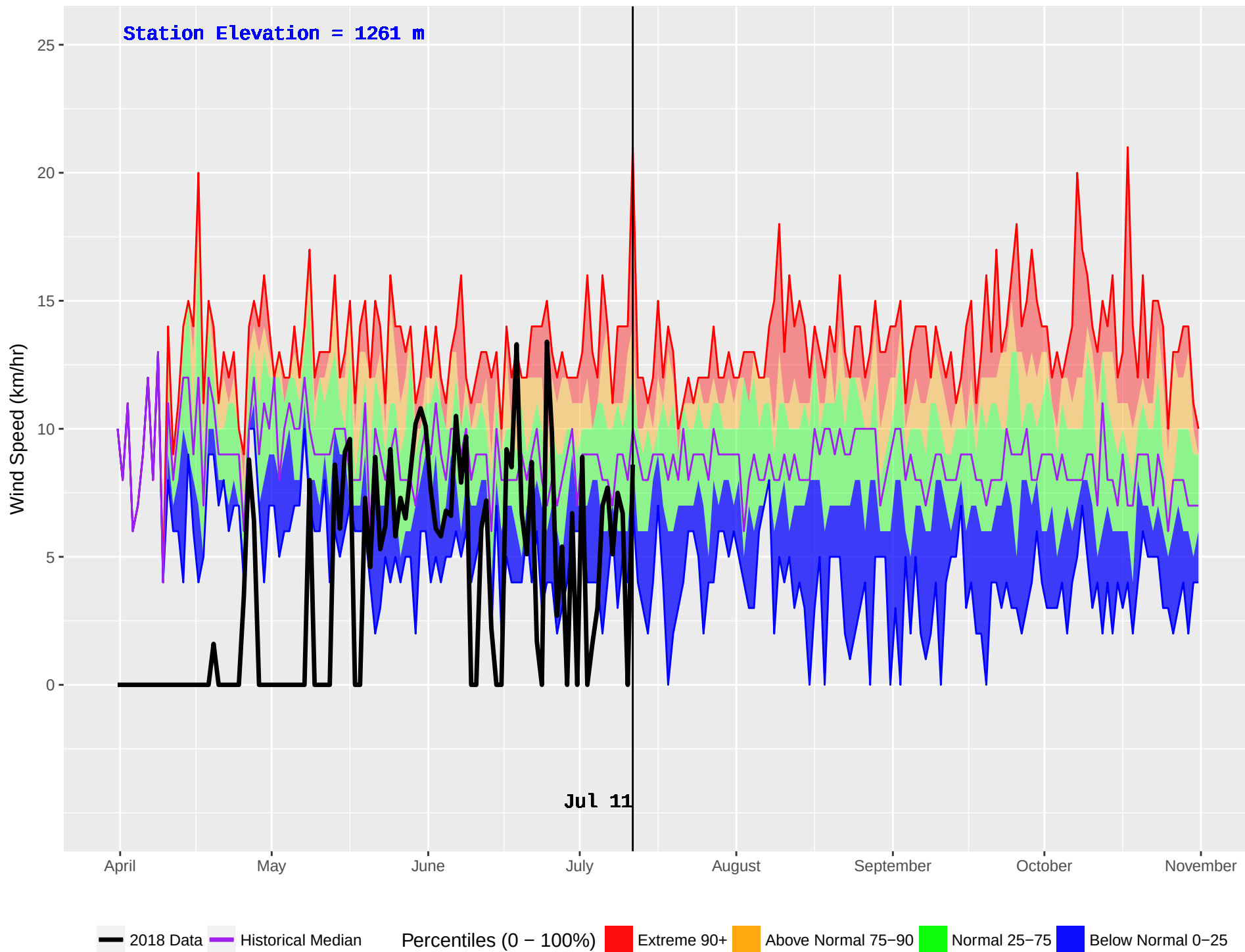
IDA BELL LAKE 3 (876) : Historical (2004–2016) and Current (2018) Noon Wind Speed
